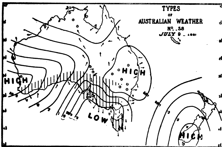
TYPE XX.—THE ADVENT OF AN ANTARCTIC STORM.
